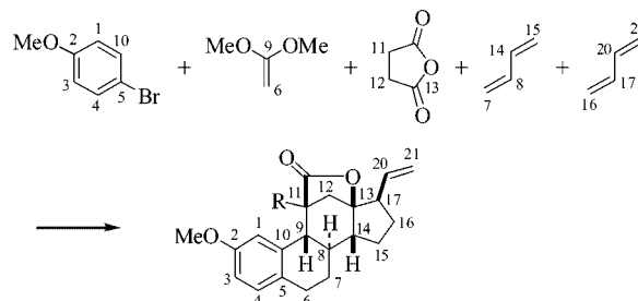
Scheme 9.
