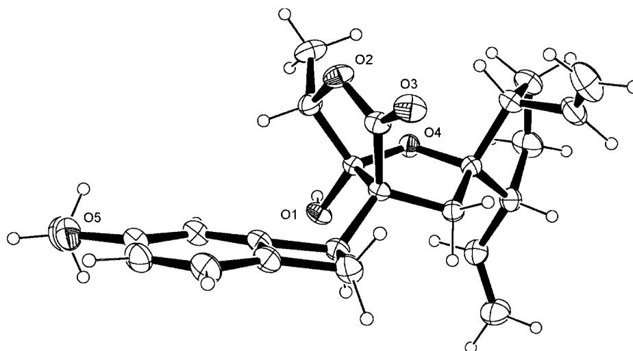
Figure 1. ORTEP diagram of compound 7 . [11]
