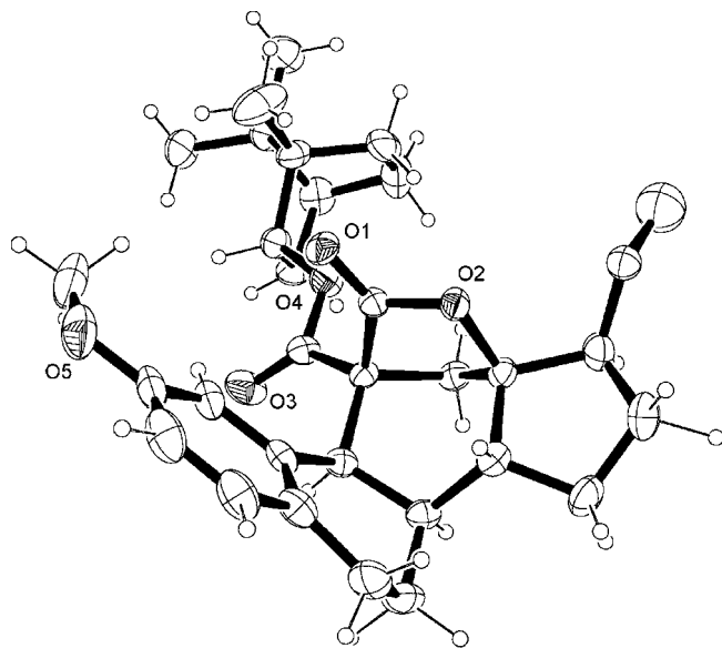
Figure 4. ORTEP diagram of steroid 15b . [19]
