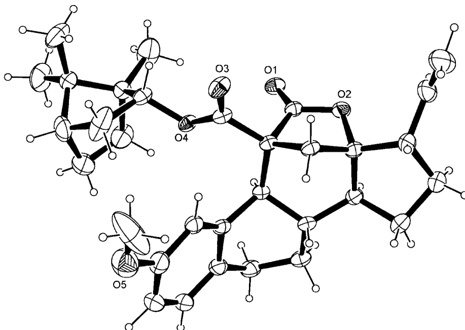
Figure 3. ORTEP diagram of steroid 14b . [11,18]
