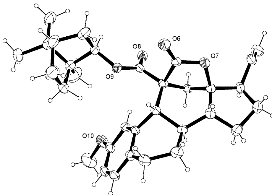
Figure 2. ORTEP diagram of steroid 13b . [11,18]
