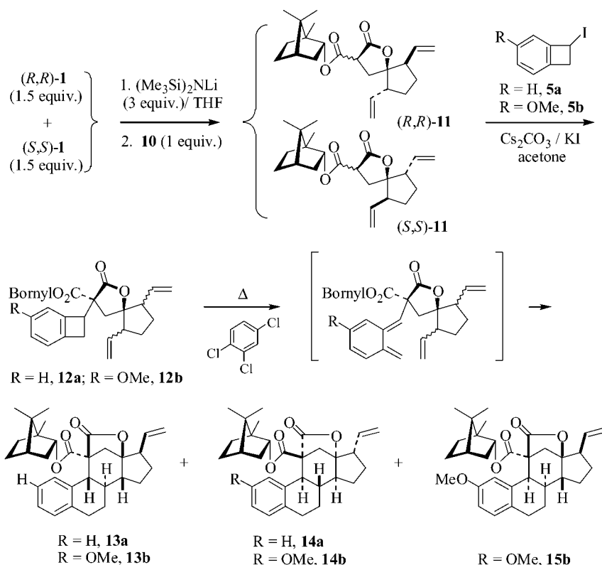
Scheme 6.
